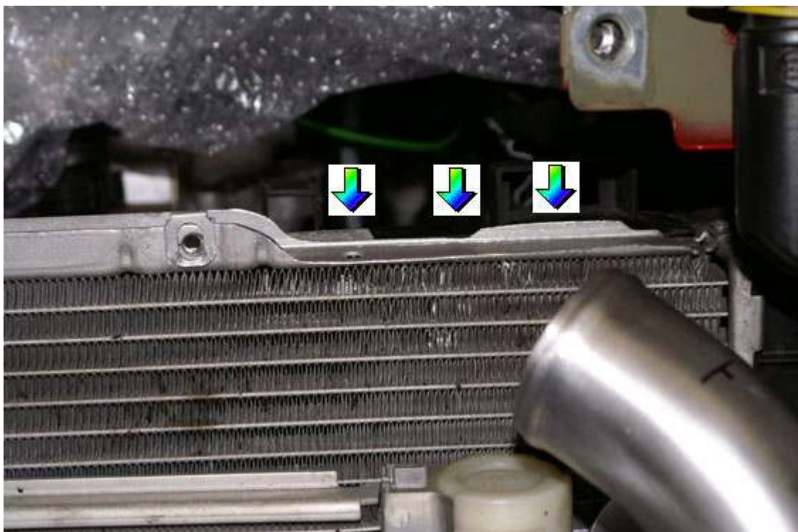
Picture 13 - Reshape top of radiator for clearance where indicated, only if required.
